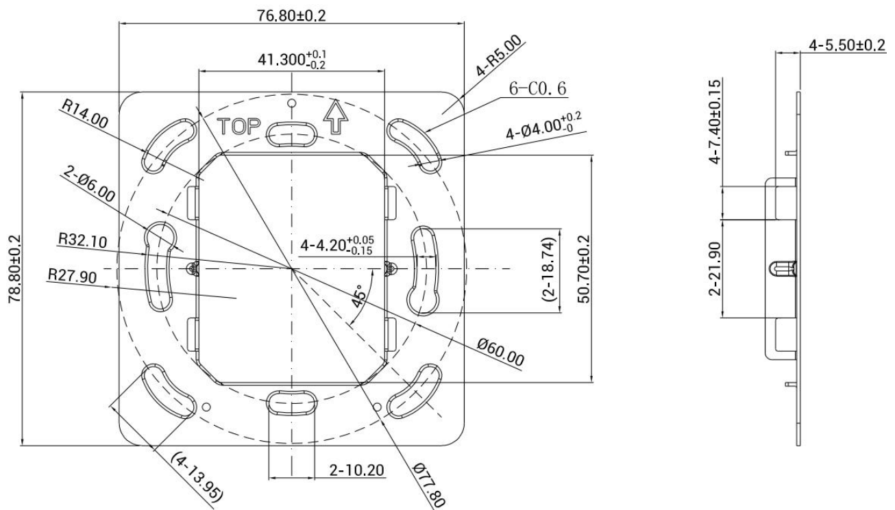
Metal plate dimension
