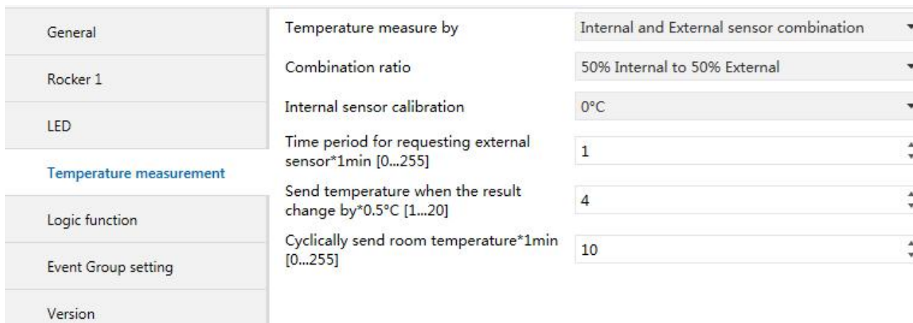
Fig. 4.16 Parameter Setting Page “Temperature measurement”
