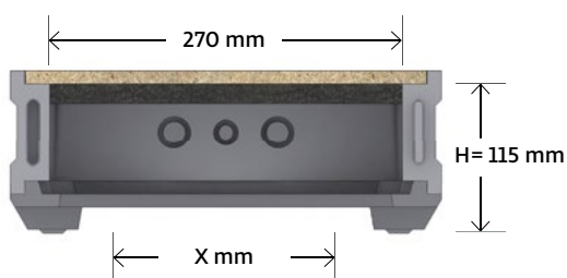
Image showing the maximum possible round cutout
