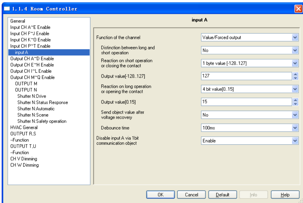
Fig. 5.6(1) parameter window “Value / Force output” (No distinction long/short operation)
