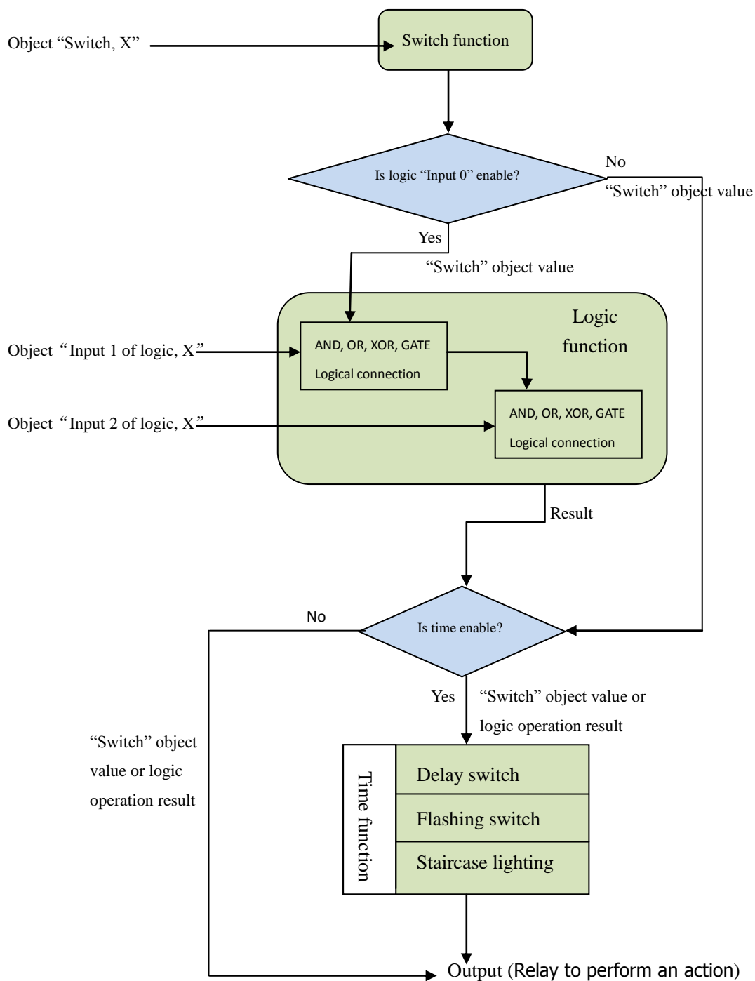
Fig. 5.10 switch, time and logical function diagram
