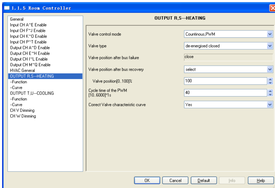
Fig. 5.35 parameter window “HEATING:Continuous, PWM”
